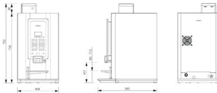
OPTIBEAN 2 (XL) NG, 3 (XL) NG SIDE VIEW RIGHT BACKSIDE All dimensions in millimeters.
